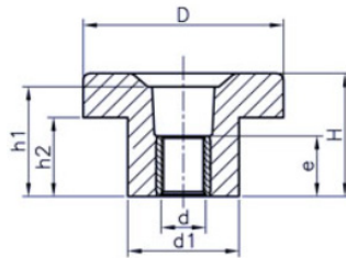
Treated Steel insert – S eg. 11- KPFB30S6
