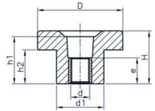
Treated Steel insert open - S eg. 11-KPFB30S6O
