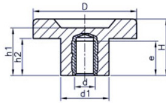
Brass insert – B eg. 11- KPFB30B6
